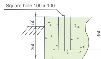
Section F-F
